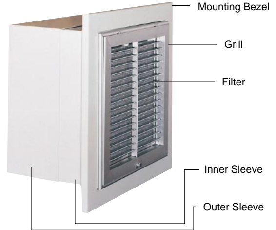
Assembled Model ADGA Angled View
