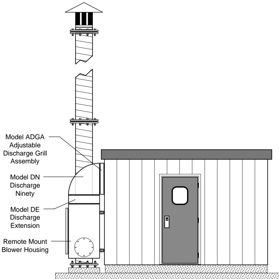
Wall Mounted Installation
