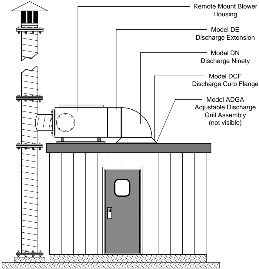
Roof Mounted Installation
